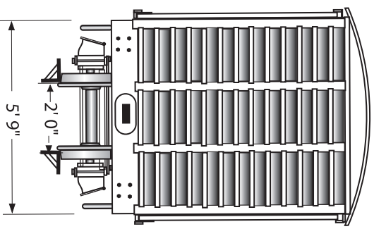
Alternative louver end on C13275
