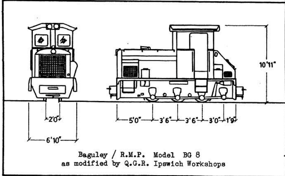
Baguley / R.M.P. Model BG 8
