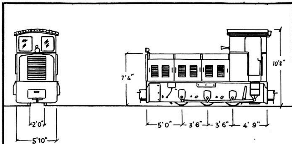
Baguley / Drewry 150hp loco.
