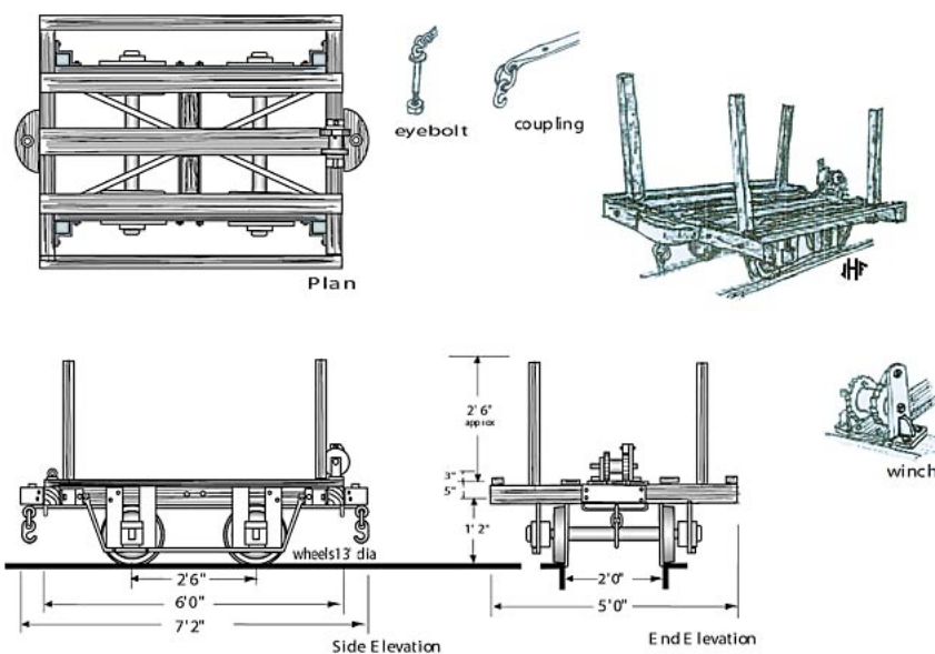
MORETON SUGAR MILL (Nambour) Whole Stick Truck
